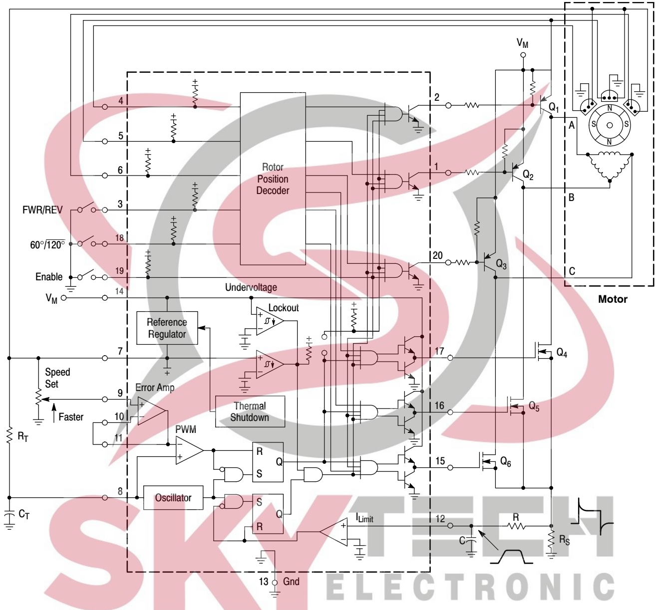
Figure 35. Three Phase, Six Step, Full Wave Motor Controller
